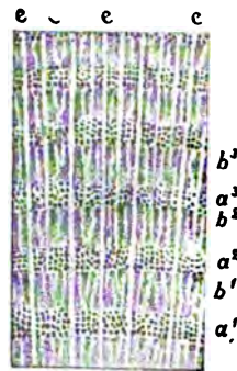
Fig. 9.—Wood of the red oak.
